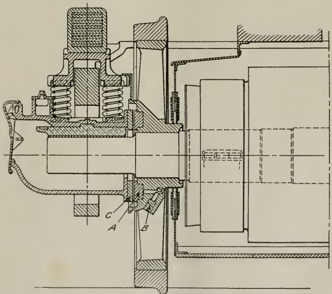
MOTOR AXLE JOURNAL BOX.
